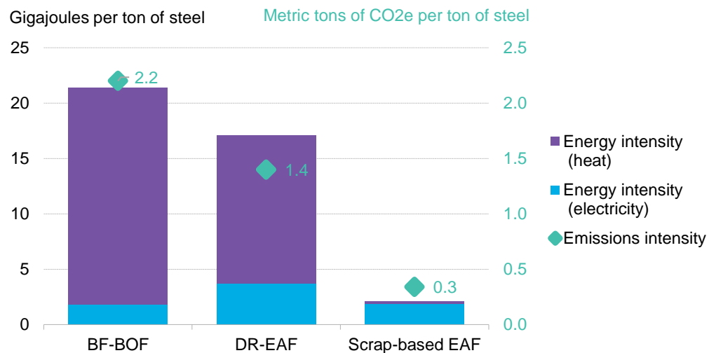
Figure 6: Energy and emissions intensities of current steel production processes
