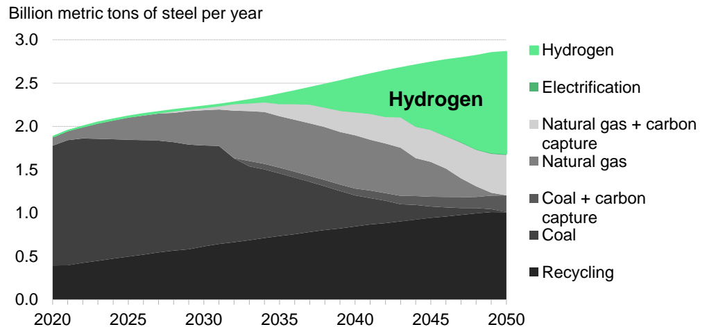
Figure 9: Pathway to net-zero emissions for global steel production in 2050, by process, in BNEF’s Net Zero Scenario
