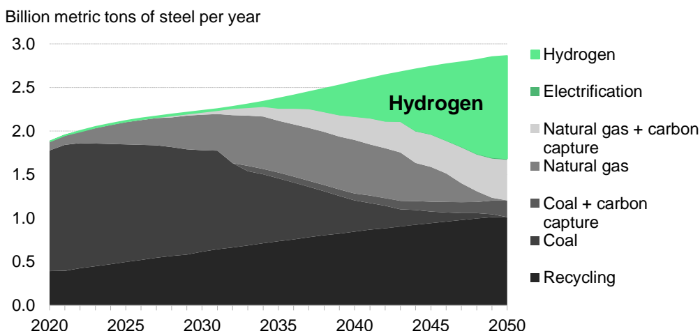
Figure 2: Pathway to net-zero emissions for global steel production in 2050, by process, in BNEF’s Net Zero Scenario
